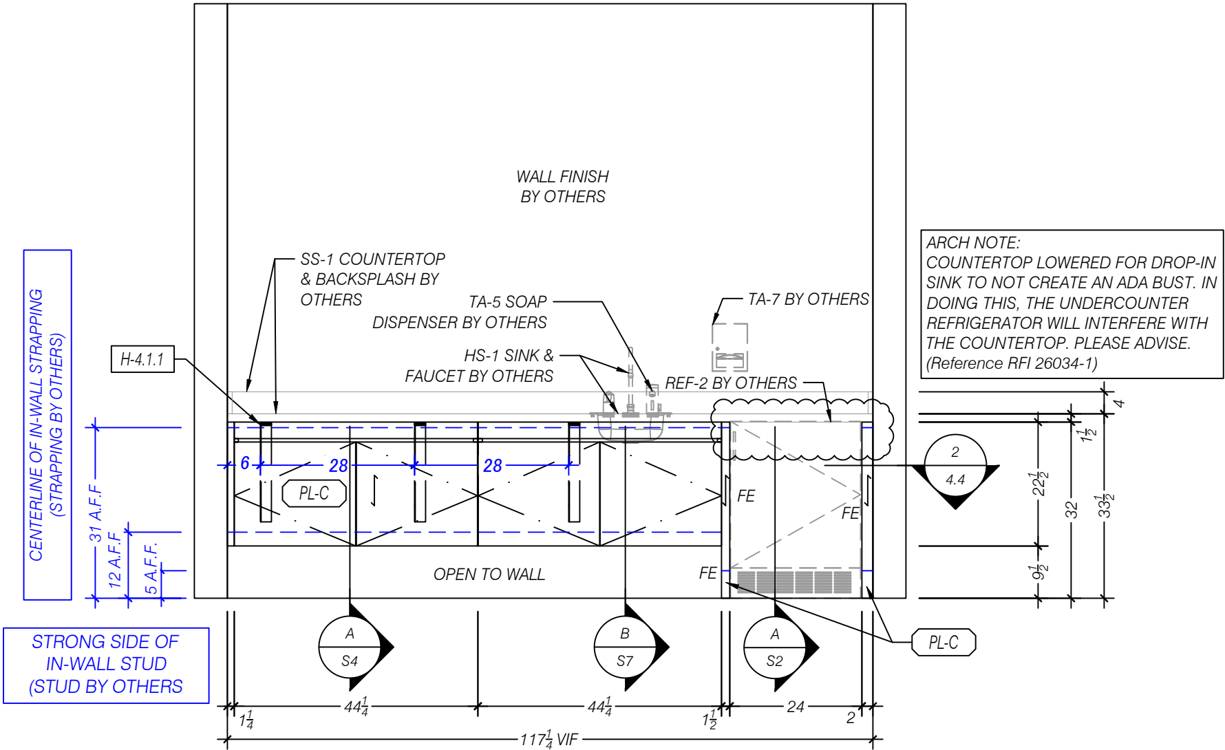
1 ELEVATION SOUTH - WELLNESS 112 SCALE 1:24 (1/2"=1'-0") ARCH REF: 13/AE406
